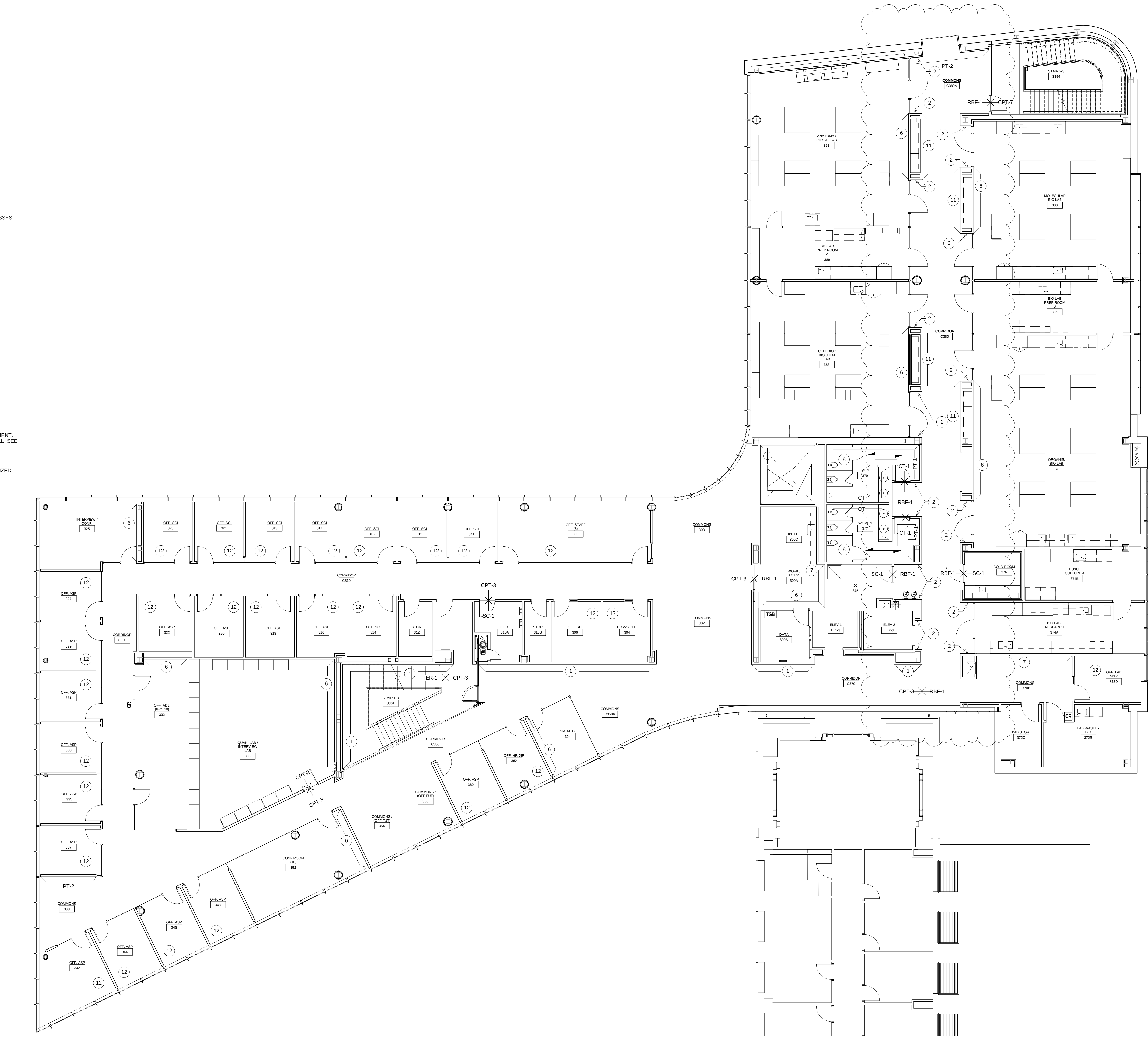
1 THIRD FLOOR TRANSITION PLAN 1/8" = 1'-0"
